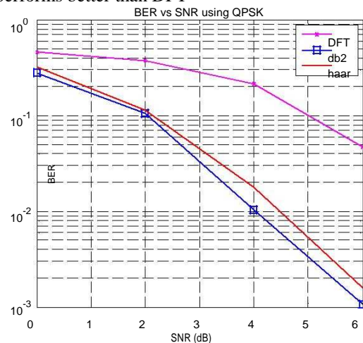
Fig. 2. BER performance of wavelets and DFT based OFDM system using QPSK modulation.
