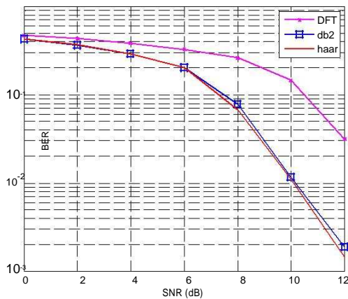
Fig. 3. BER performance of wavelets and DFT based OFDM system using 16-QAM technique.
