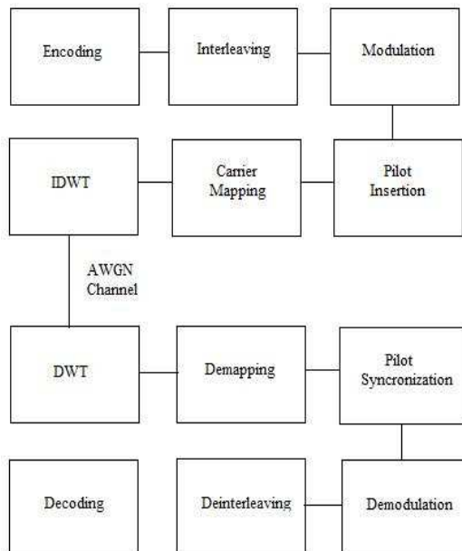
Fig. 1. Block diagram of Wavelet based proposed OFDM system design.
