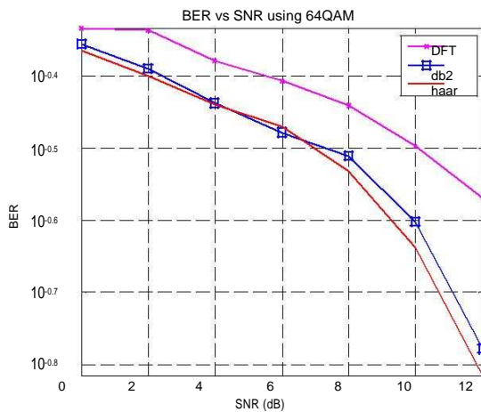
Fig. 4. BER performance of wavelets and DFT based OFDM system using 64-QAM modulation.
